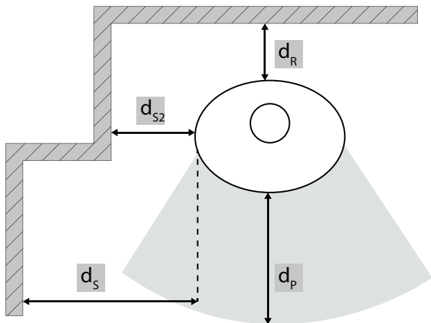
LOKI distance to combustible materials; position layout 1C
